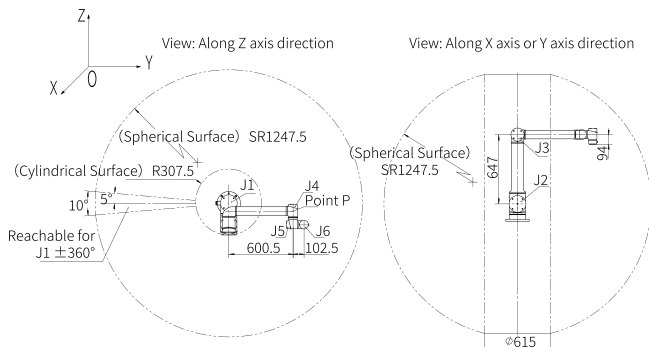
WORKSPACE DIMENSIONS
