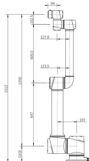
PRODUCT DIMENSIONS
